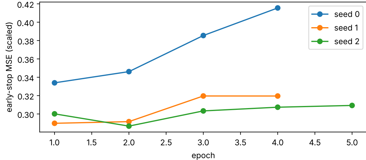
Early stopping
